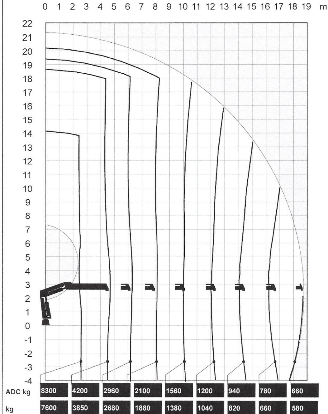
Load diagram
